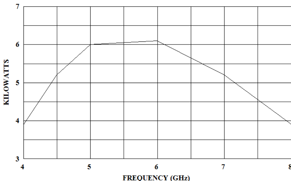
4000TP4G8 Typical Peak Pulse Power Output
